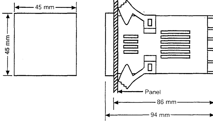
Figure 6.1 Mounting Dimensions
